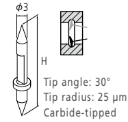
Double-sided conical stylus
