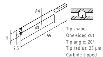
Small hole stylus SPH-43
