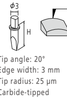
Small hole stylus SPH-41
