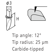
One-sided cut stylus
