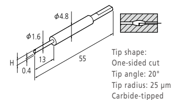
Small hole stylus SPH-41
