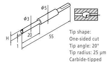
Small hole stylus SPH-43
